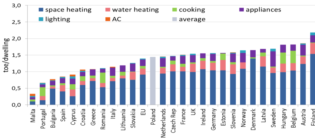
Figure 42: Breakdown of household energy use by end-use (2012)
