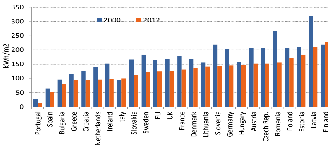
Figure 45: Energy use for space heating per m 2 33
