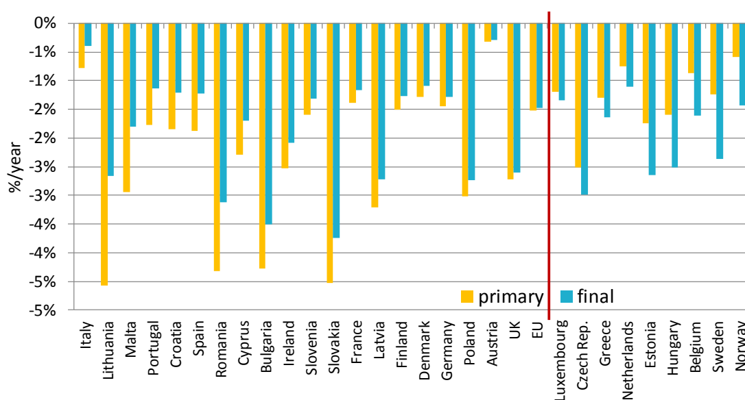
Figure 6: Variation of primary and final energy intensities in EU countries 8
