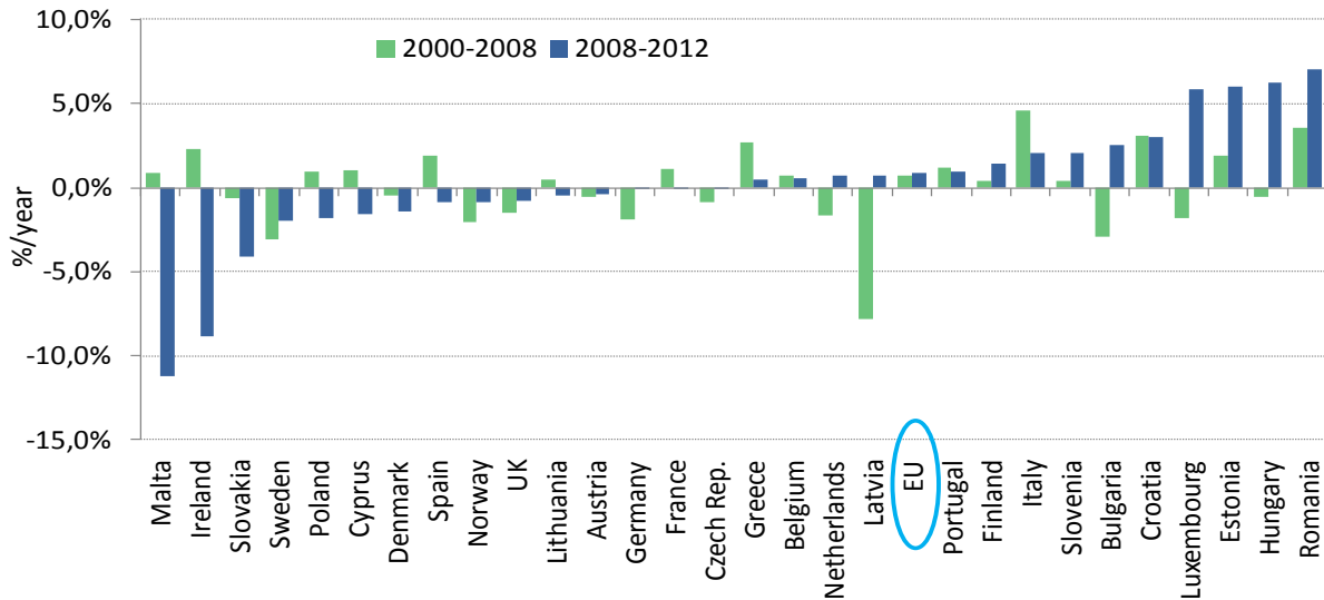
Figure 56: Electricity intensity trends in services
